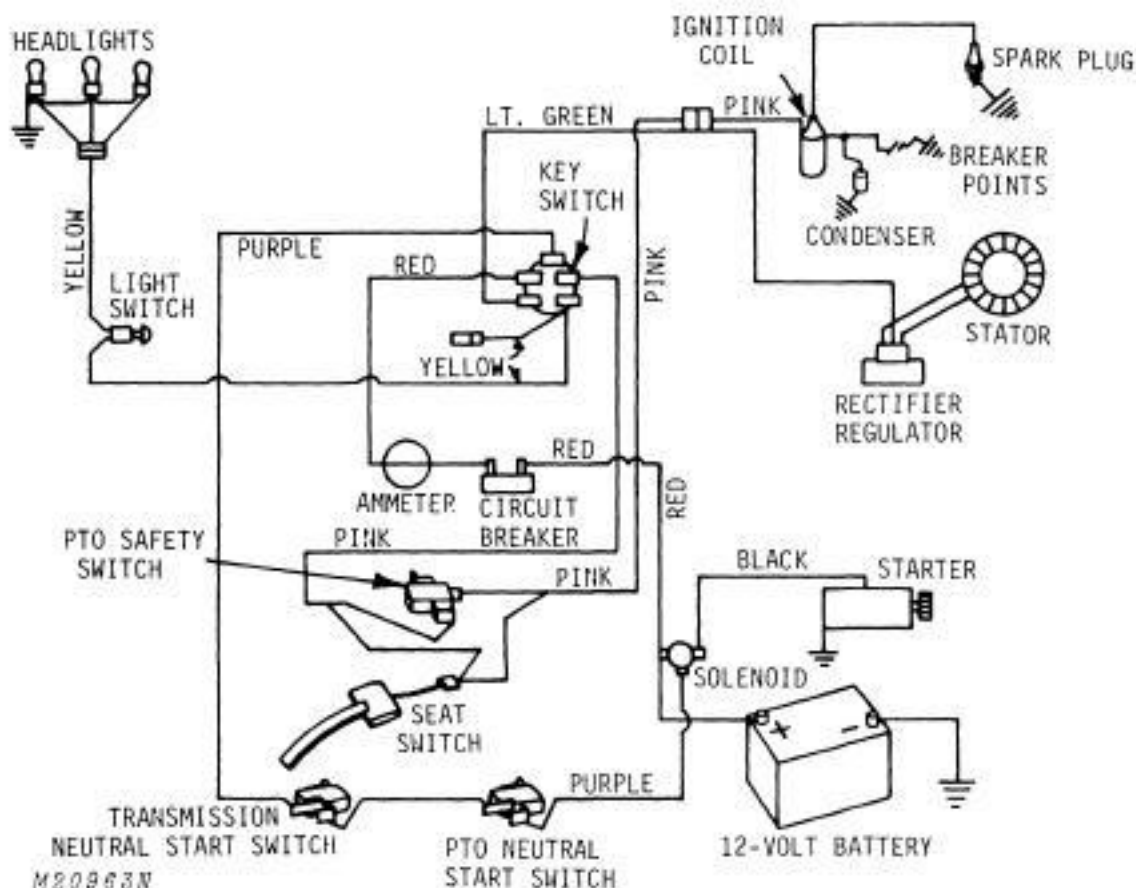
Fig. 3-Wiring Diagram For 210, 212, 214 and 216 Tractors (Serial No. 70,001-190,000)
