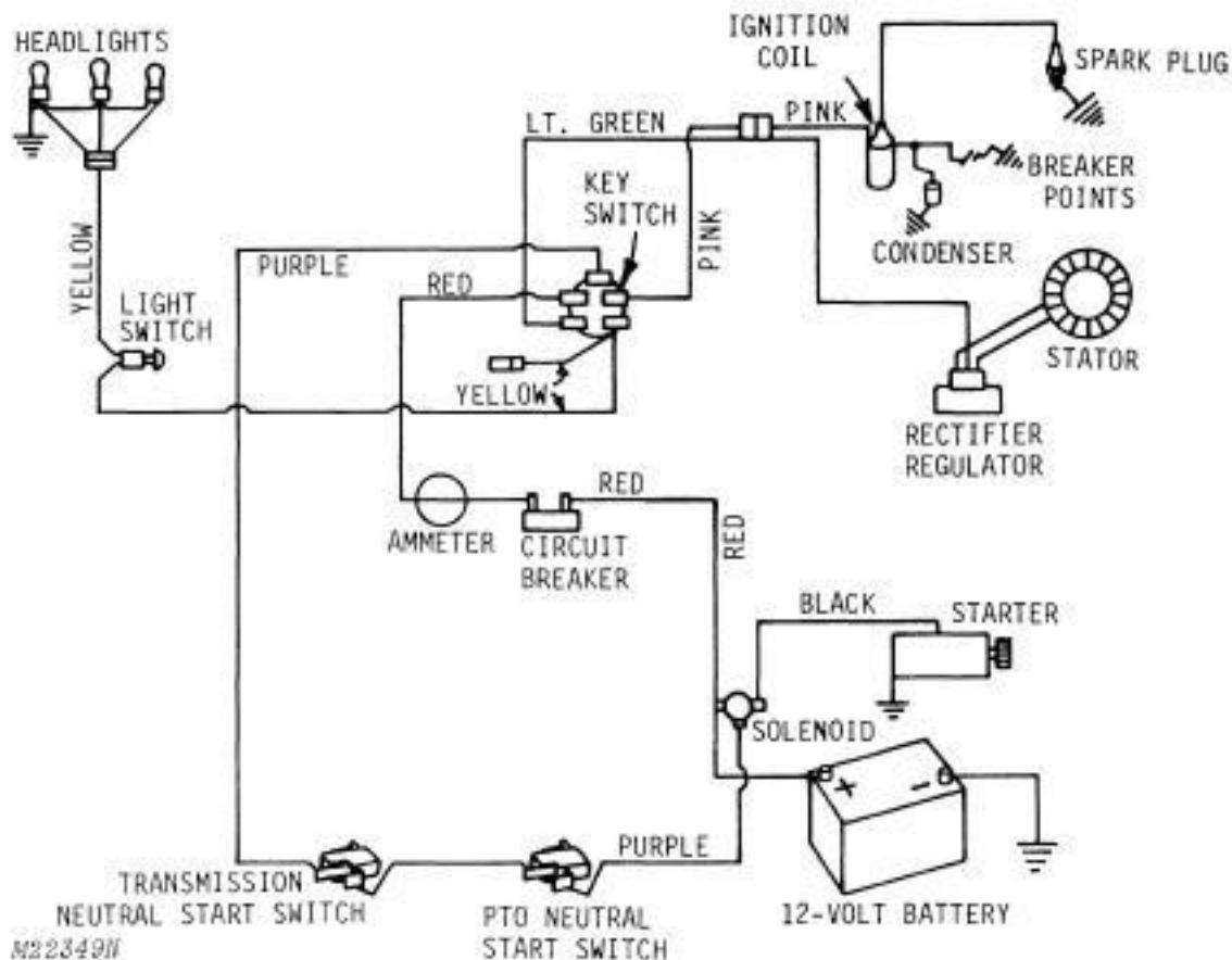
Figure 1-Wiring Diagram For 200, 210, 212 and 214 Tractors (Serial No. 30,001-70,000)
