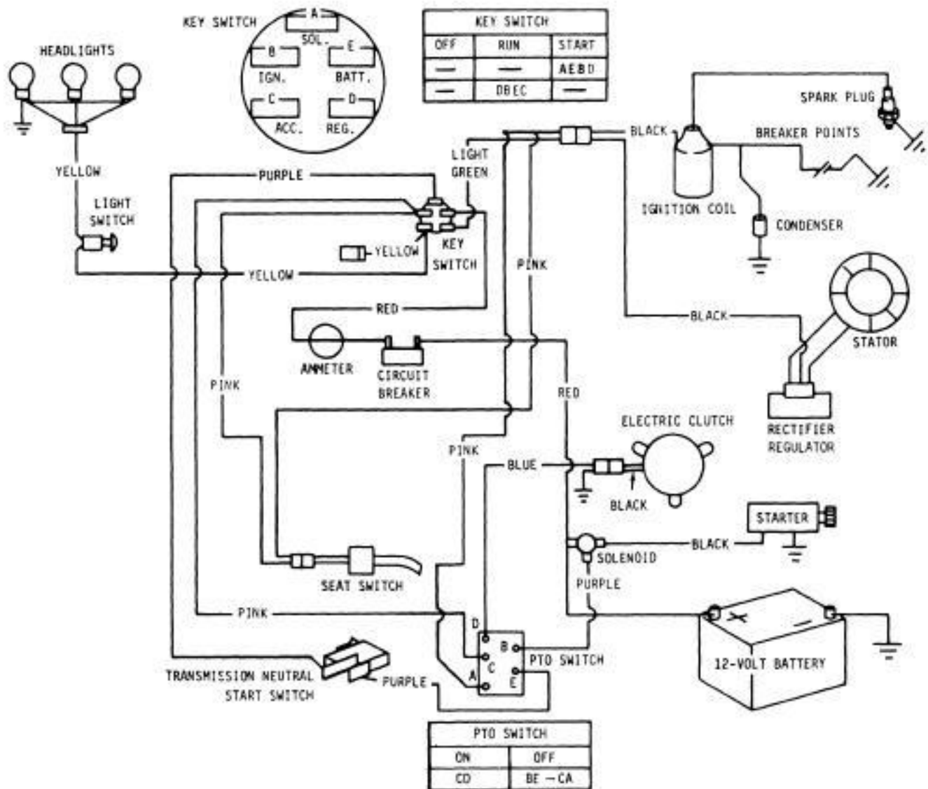
Fig. 4-Wiring Diagram For 210, 212, 214 and 216 Tractors (Serial No. 190,001- )
